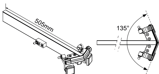
Scatola 087 AAP completa 45°, L=505 SQ Compl. 087 45° Open Corner case L=505 SQ
